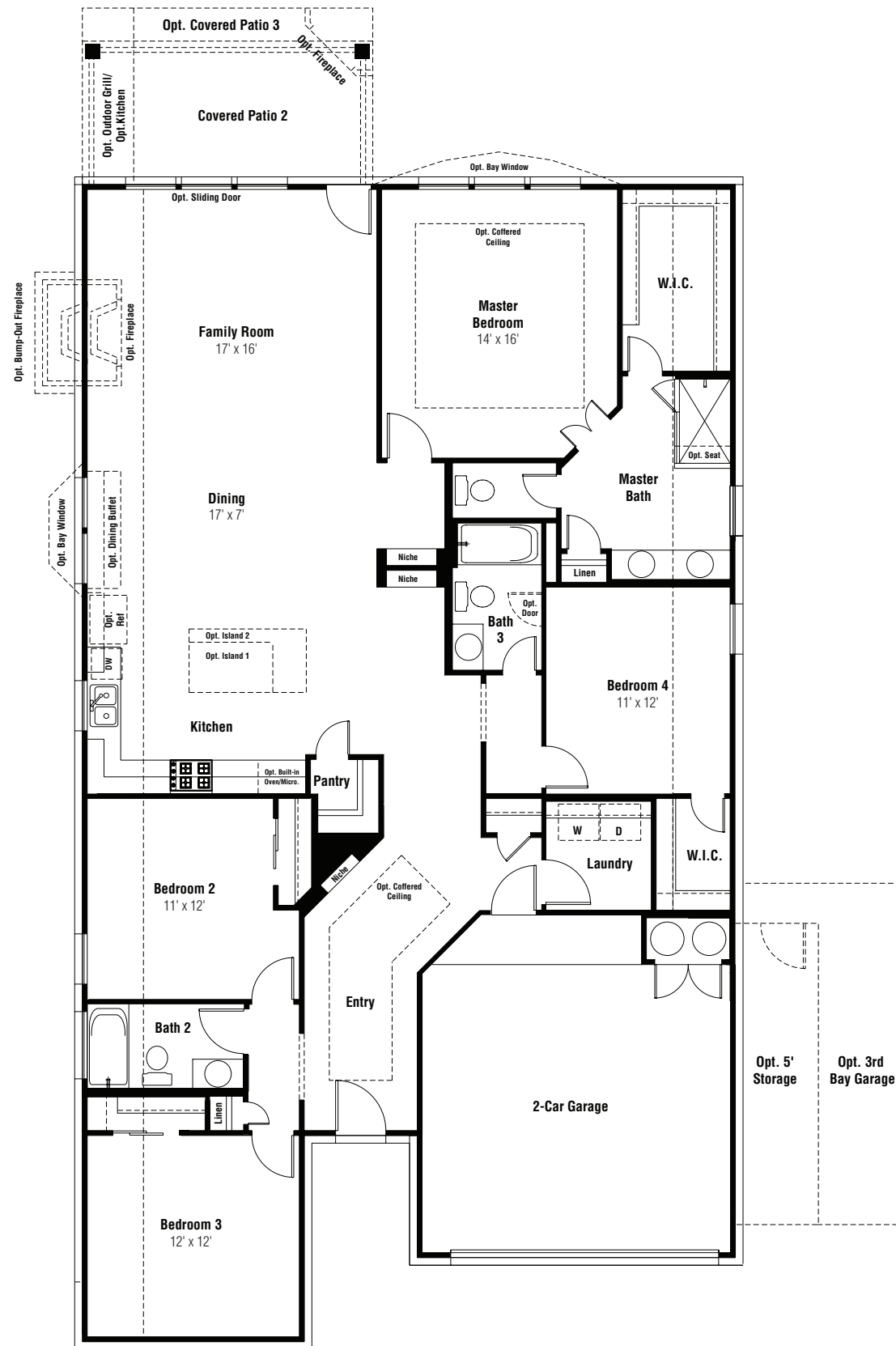
FIRST FLOOR
