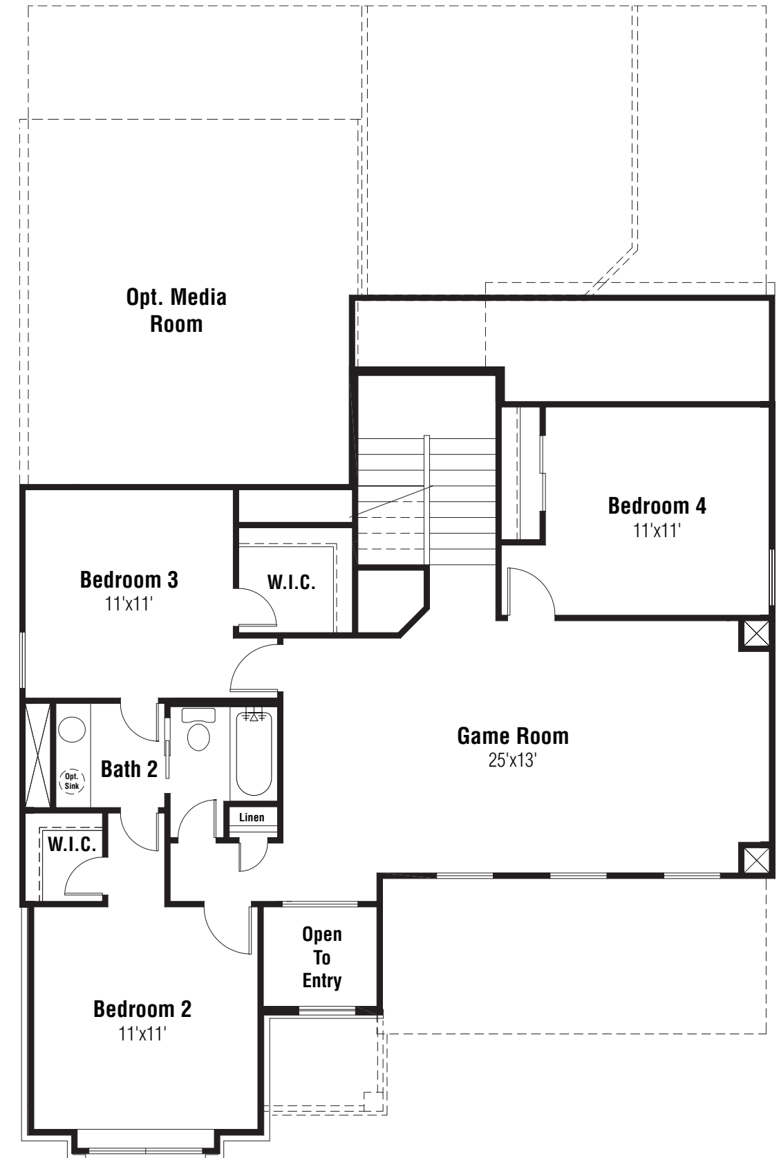
SECOND FLOOR
