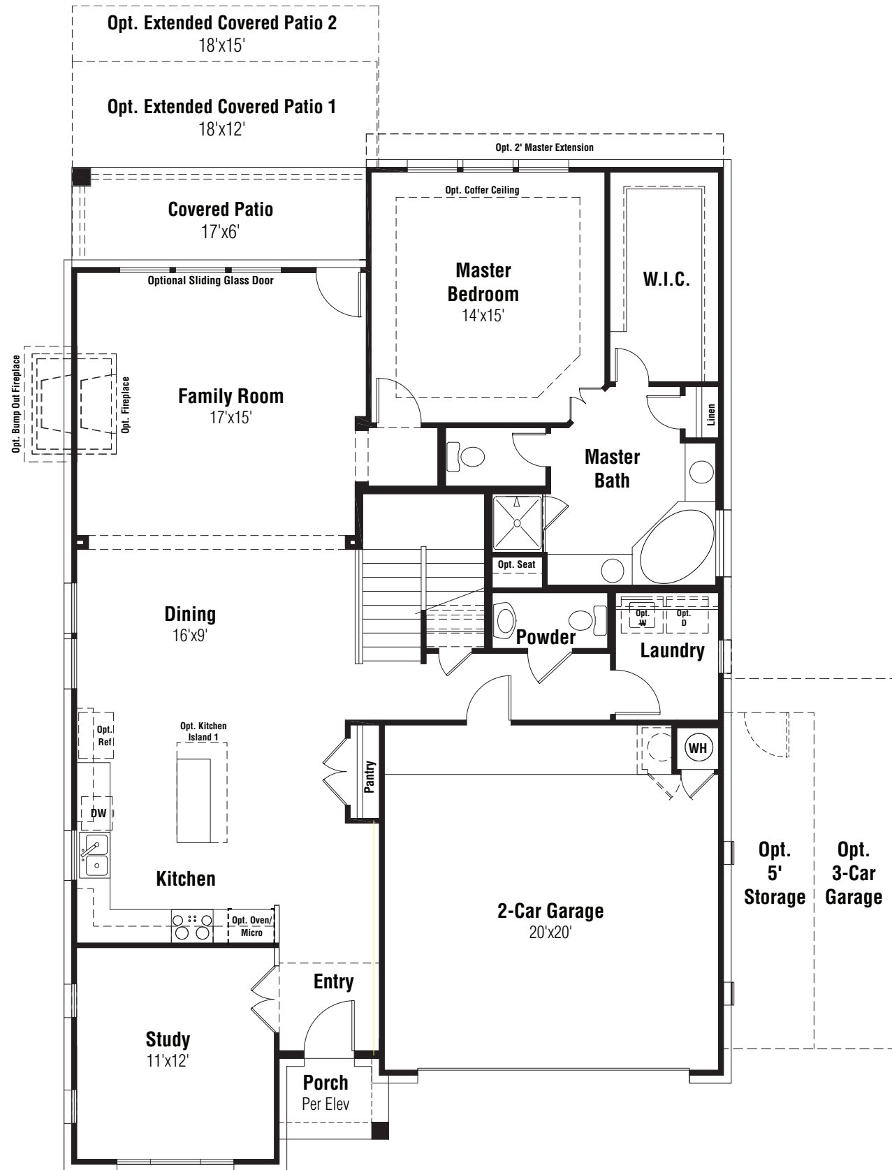
FIRST FLOOR
